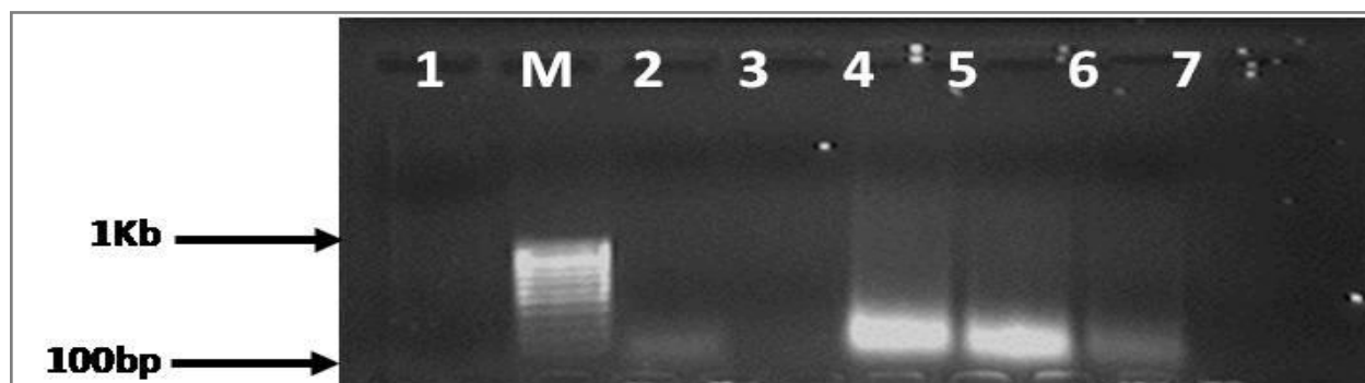
Figure 6. DNA extracted from scat samples of carnivores using Qiagen kit on 0.8 % agarose gel. M, MW marker 100bp ladder.
